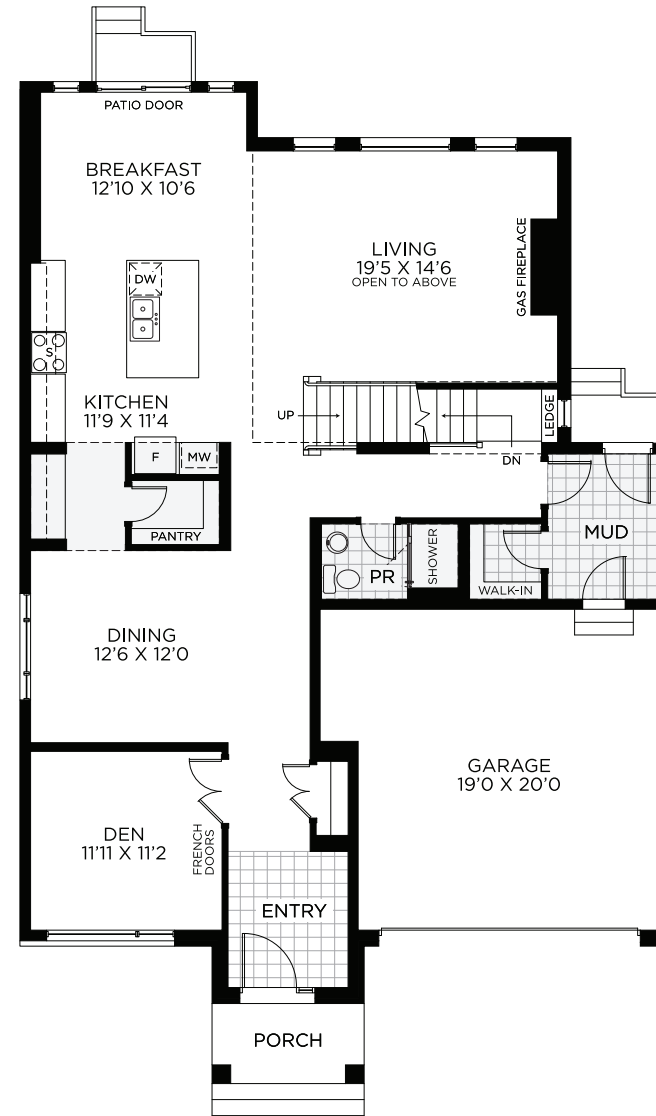
OPT. GROUND FLOOR 3PC Powder Room
