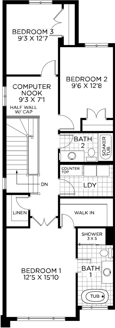
BEDROOM FLOOR
